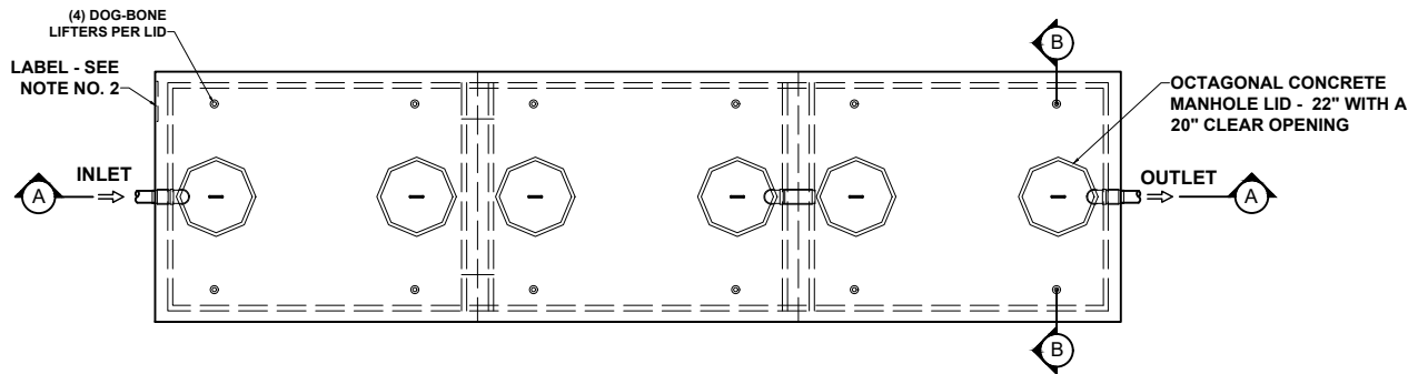
PLAN VIEW
